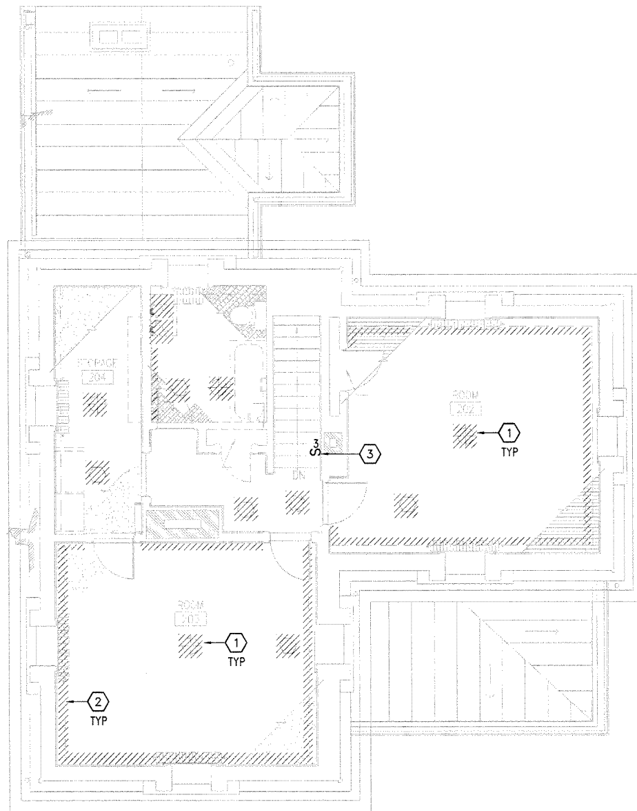
1 ED1.02 SECOND FLOOR DEMOLITION PLAN SCALE: 1/4" = 1'-0"
