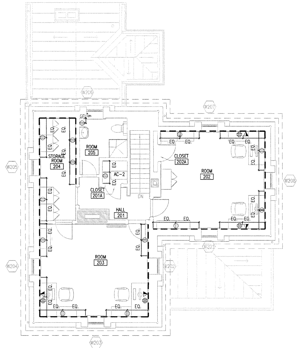
1 SECOND FLOOR POWER PLAN A8.02 1/4"=1'-0"
