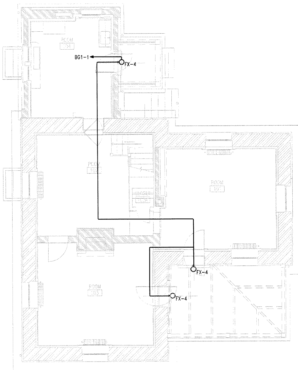
2 FIRST FLOOR LIGHTING PLAN E1.01 SCALE: 1/4" = 1'-0"
