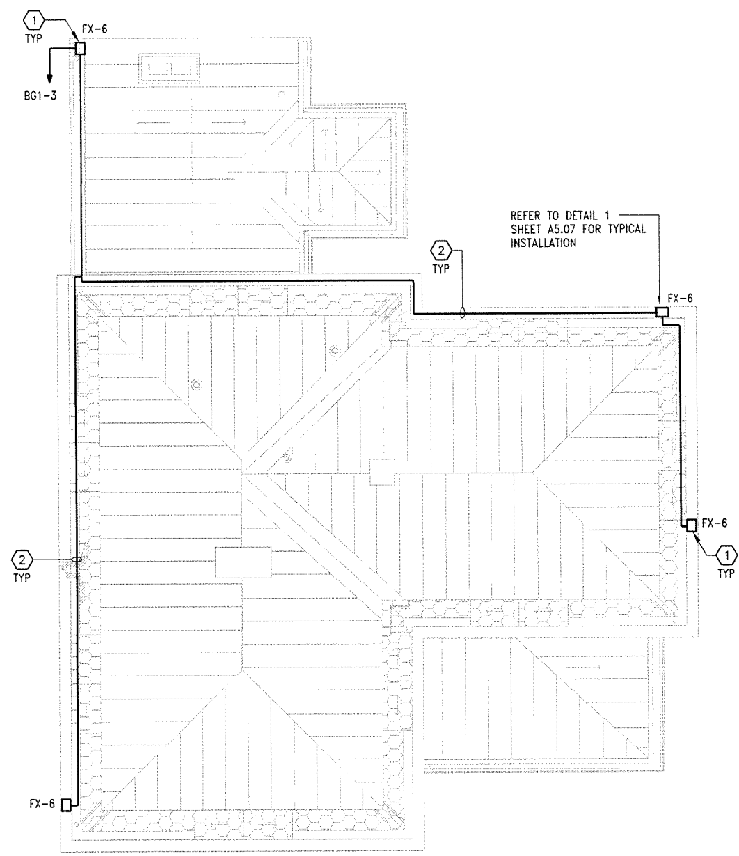
2 ROOF LIGHTING PLAN E1.01 SCALE: 1/4" = 1'-0"
